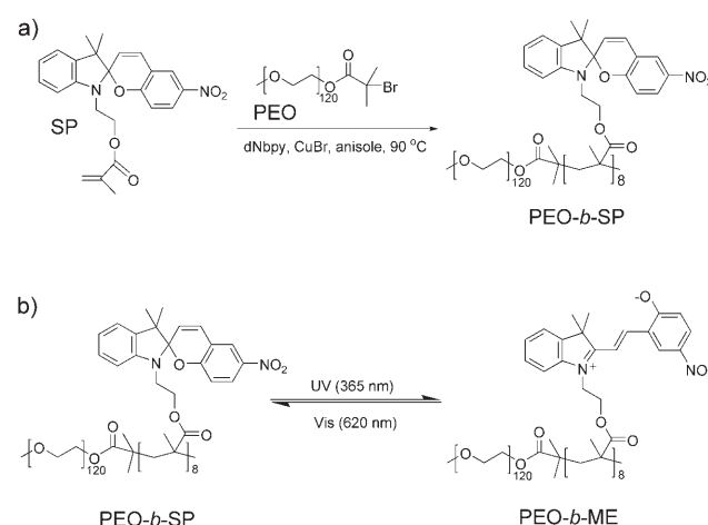
Scheme 1. a) Synthesis of a PEO-b-SP diblock copolymer; dNbpy = 4,4'-bis(5-nonyl)-2,2'-bipyridine. b) Light-induced isomerization between PEO-b-SP (colorless aqueous solution) and PEO-b-ME (purple aqueous solution) by alternating irradiation of UV and visible light.
